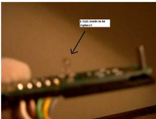
Use soldering iron to remove the bulb and replace.
